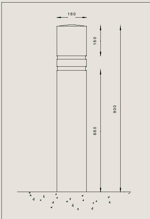
GATESHEAD BOLLARD MOUNTED ON LOCKABLE REMOVABLE ADAPTOR
