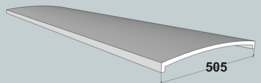
CAPPING ARCH 505
