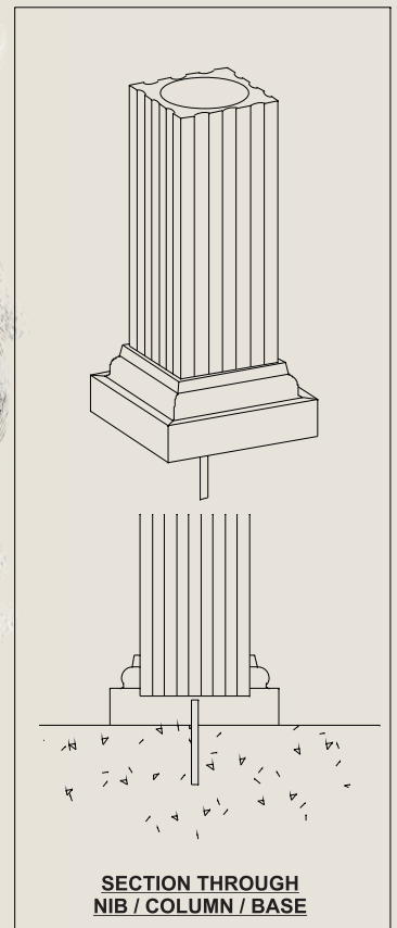
PERMAPOST COLUMN WITH CAPITAL & BASE
