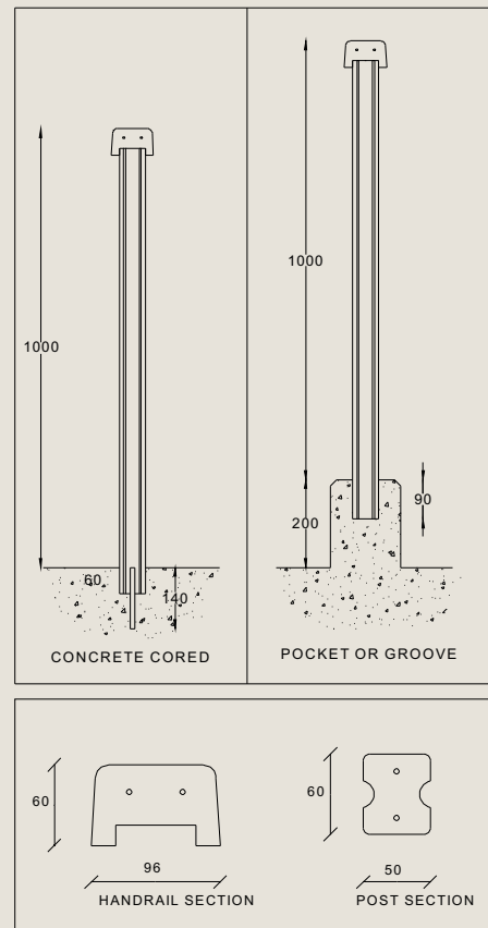
NATIONAL ROADS 4.5 Kn/m LOADING
